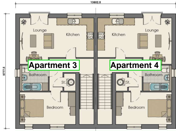
Norbury House - First Floor
