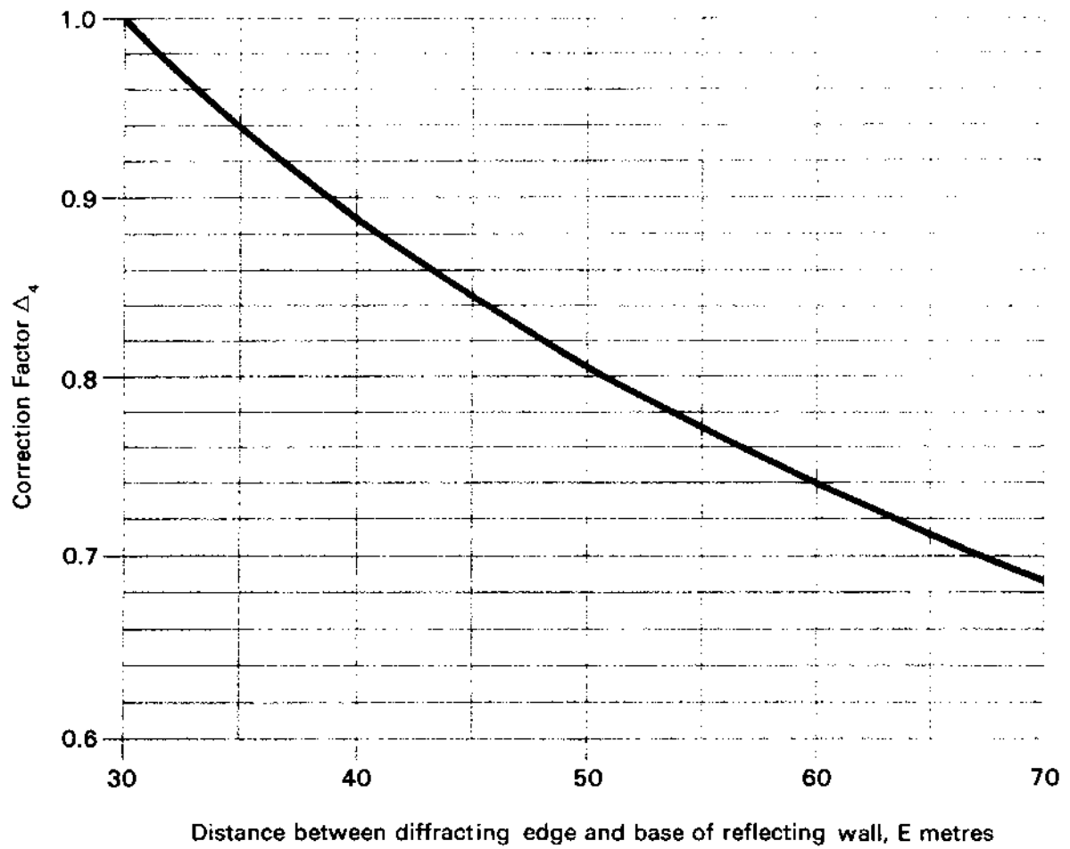
Chart 14 CORRECTION FACTOR \Delta_4 IN TERMS OF DISTANCE, E. [To be used in conjunction with Charts 13 and 15]
