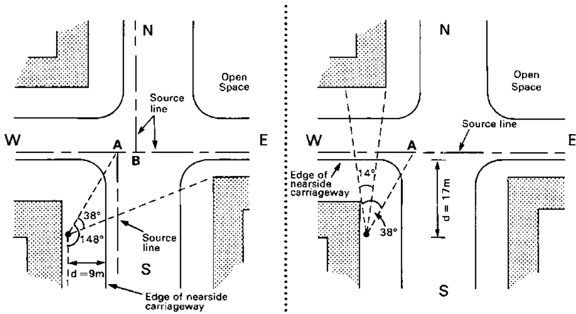
(i) Segment S: d = 9\text{m} Angle of view = 148^\circ Angle of reflection = 148^\circ - 38^\circ = 110^\circ
